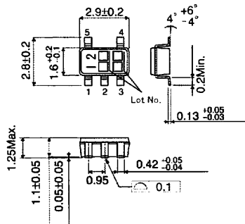
BU4S01G2(SSOP5)(UNIT:[mm])
